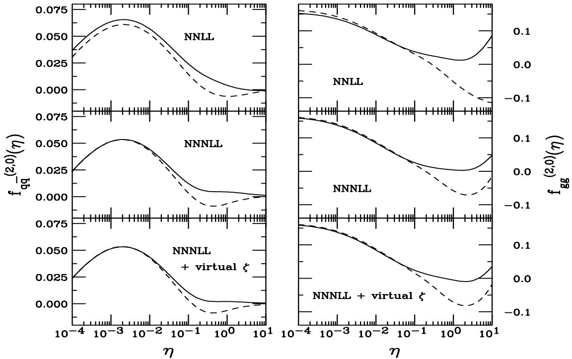
Fig. 1. The f_{ij}^{(2,0)} scaling functions in the \overline{\text{MS}} scheme for the q\bar{q} (left) and g\bar{g} (right) channels. The top plots show the NNLL result, the center plots the NNNLL results and the bottom plots give the results including the virtual \zeta terms. The solid curves are for 1PI kinematics, the dashed for PIM kinematics
