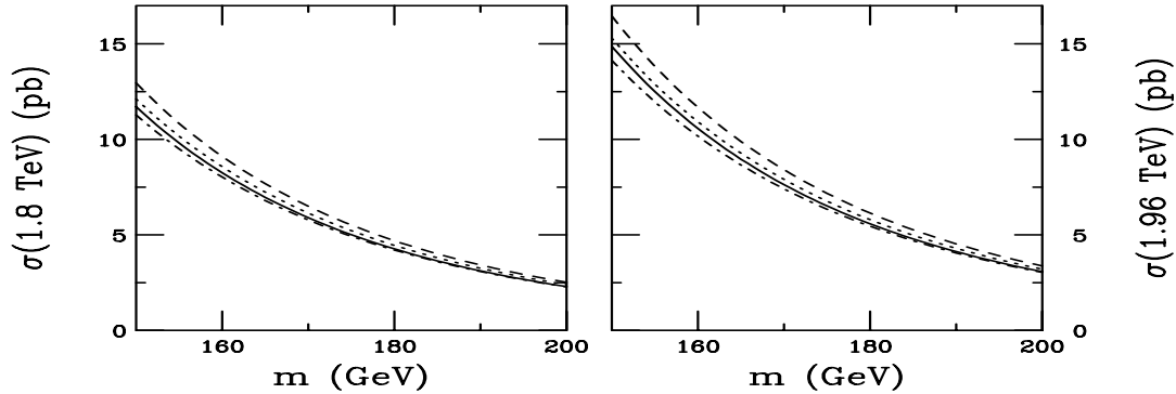
Fig. 2. The t\bar{t} total cross sections in p\bar{p} collisions at \sqrt{s} = 1.8 TeV (left-hand side) and 1.96 TeV (right-hand side) as functions of m for \mu = m . The NLO (solid), and approximate NNLO 1PI (dashed), PIM (dot-dashed) and average (dotted) results are shown
